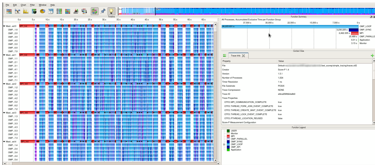
Fig. 3: Vampir window
